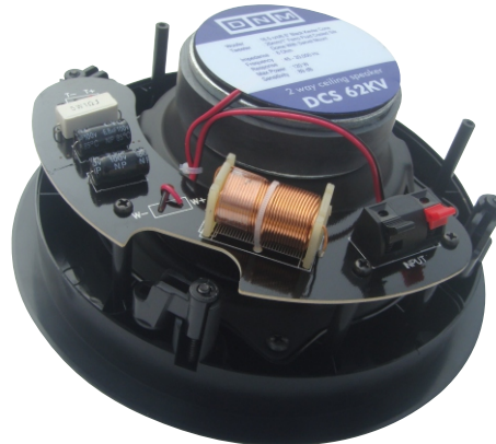
REAR VIEW OF DCS 62KV SPEAKER WITH LARGE WOOFER MAGNET 90mm x 17mm, HIGH PERFORMANCE CROSSOVER AND DOG EARS FOR MOUNTING
